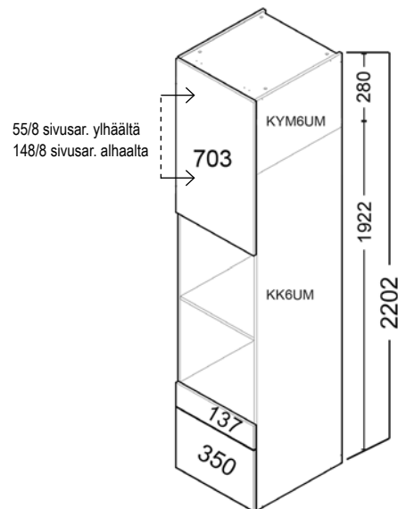
KK6UM + KYM6UM 703 MM OVELLA
